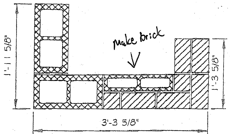
Plan Sect. at Starter Course
