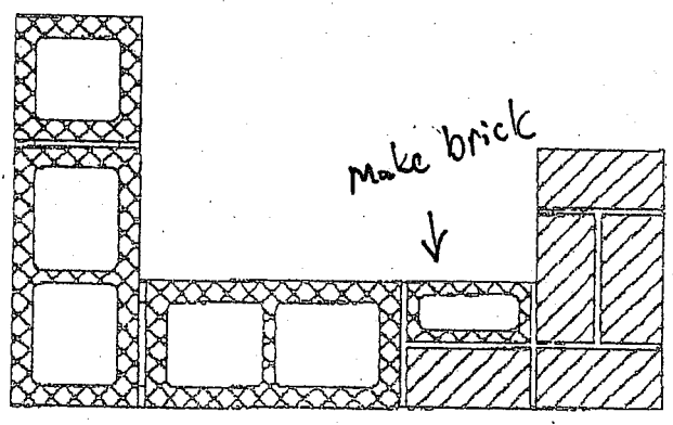
Plan Sect. at 2nd Block Course
