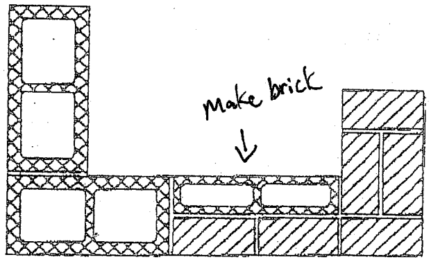
Plan Sect. at 2nd Brick Course
