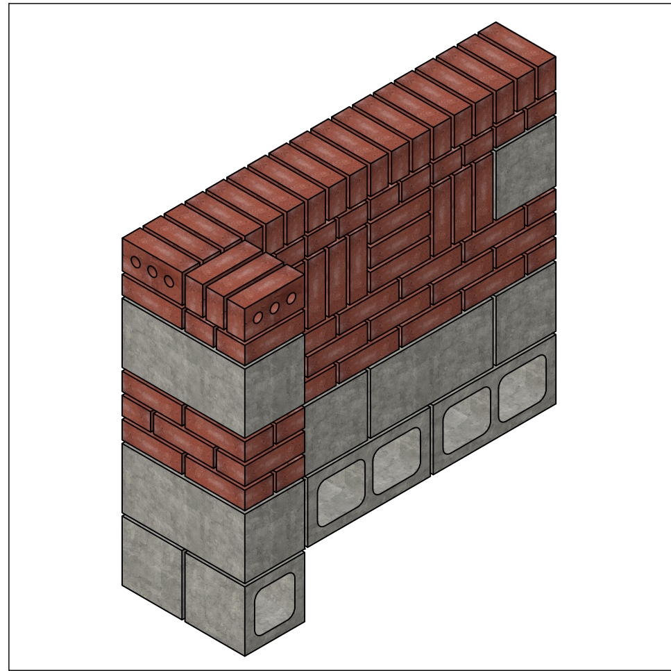
1. ISOMETRIC VIEW
