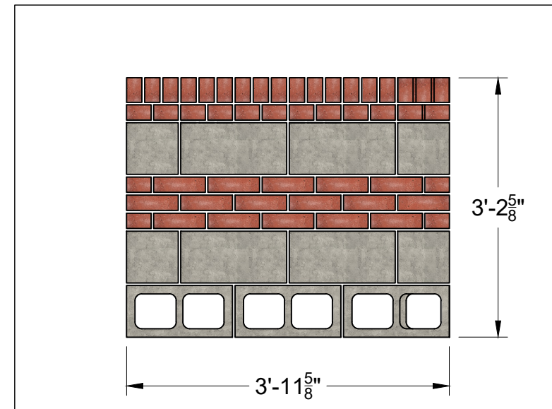
5. BACK ELEVATION
