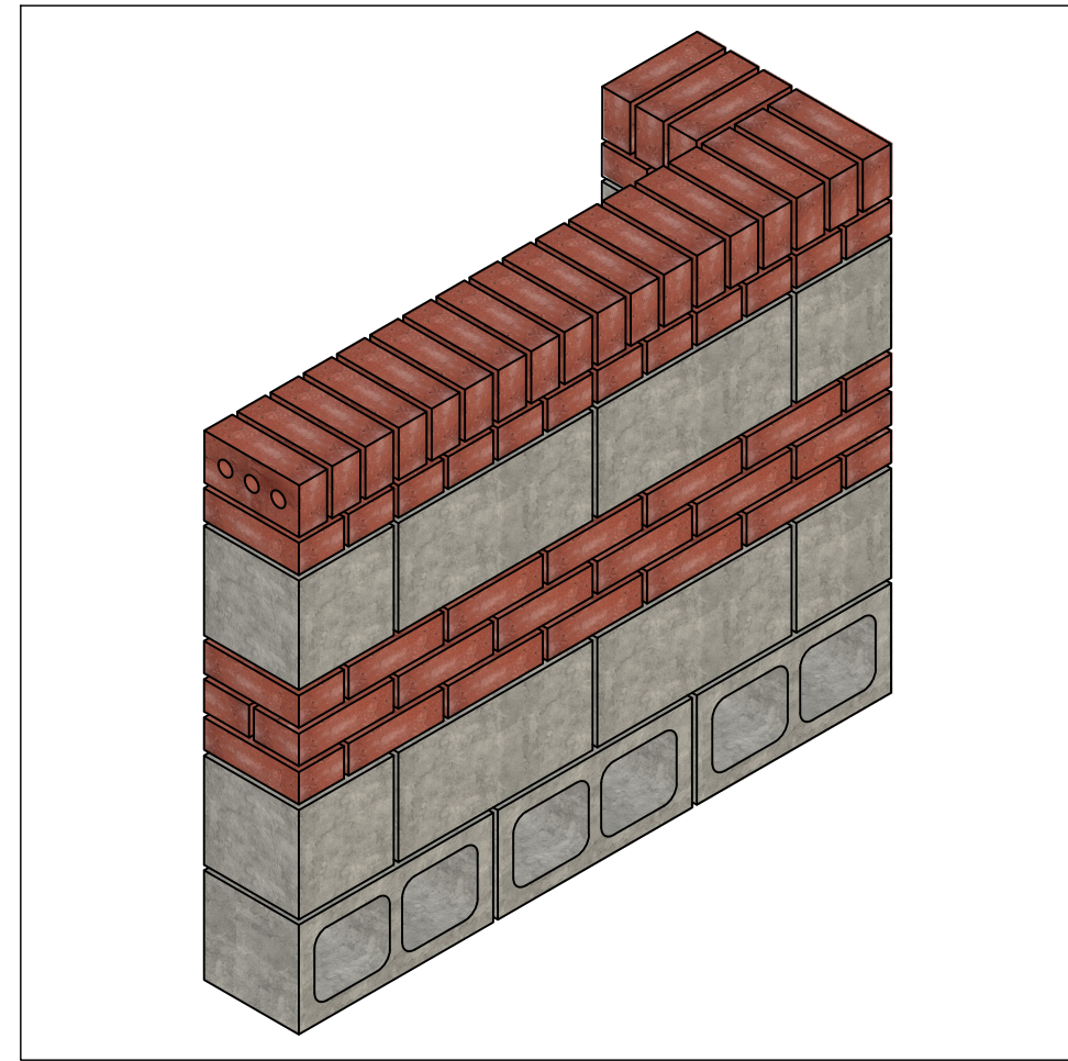
2. ISOMETRIC VIEW
