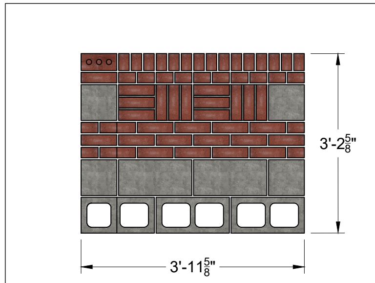
4. FRONT ELEVATION
