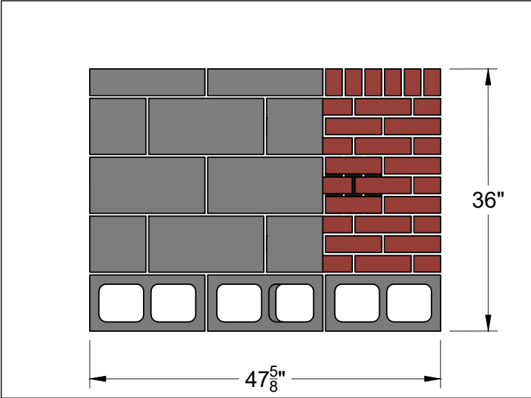
5. BACK ELEVATION
