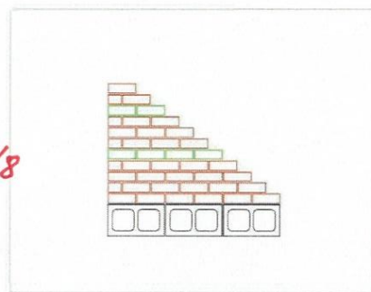
3 FRONT ELEVATION SCALE 1/4" = 1'-0"
